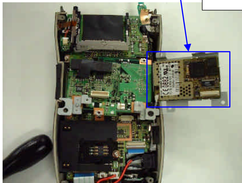
MC46 Module Adapter Position
