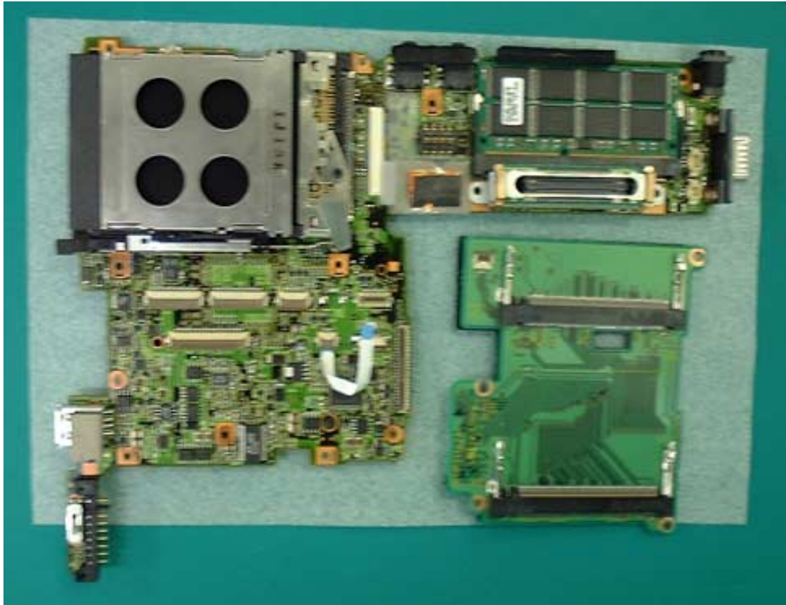
Main PCB Top View
