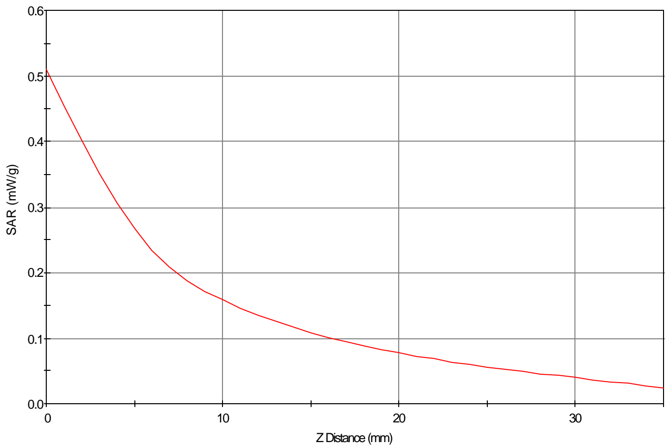
SAR - Z Axis at Hotspot x:-7.0 y:14.0
