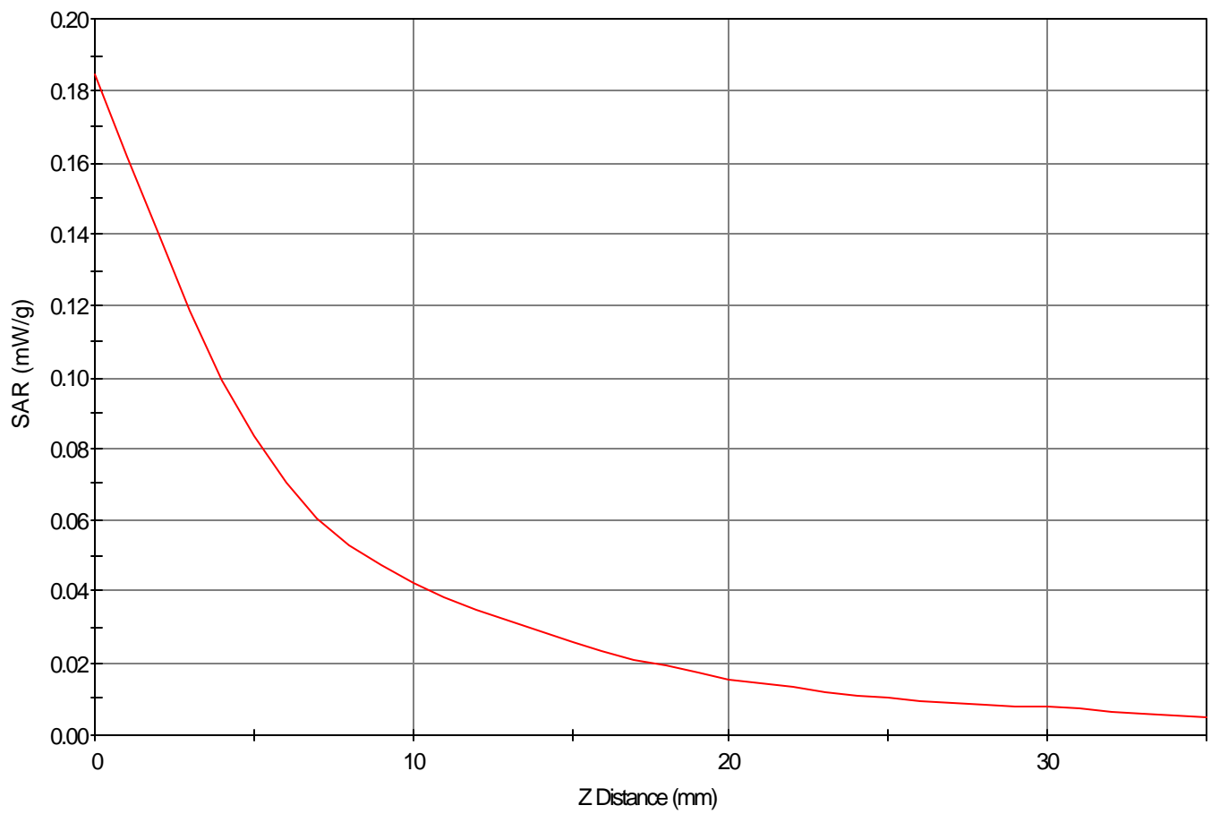
SAR - Z Axis at Hotspot x:-11.0 y:5.0
