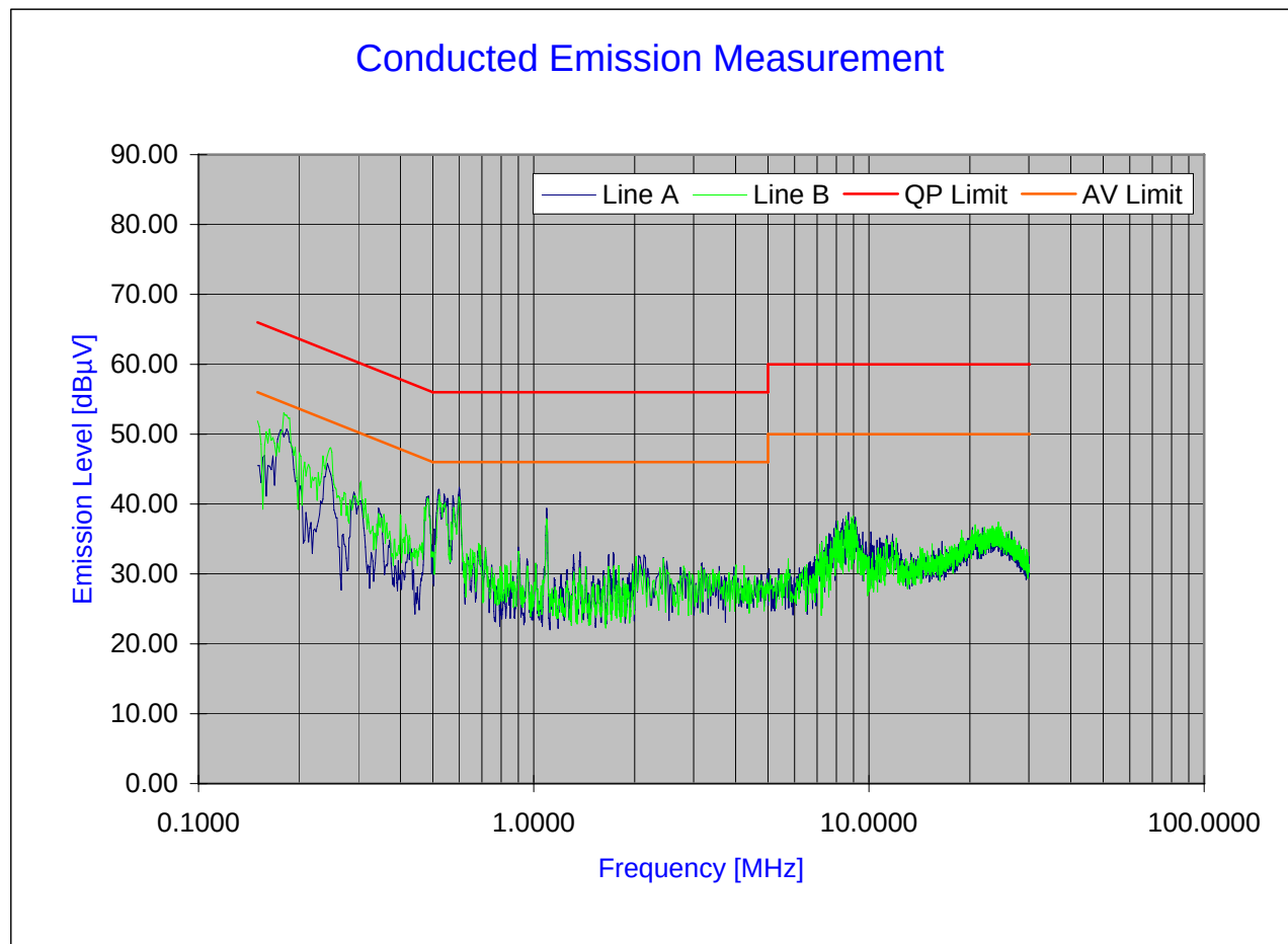
Plot 6-27. Line Conducted Plot with 802.11a with Docking Station
