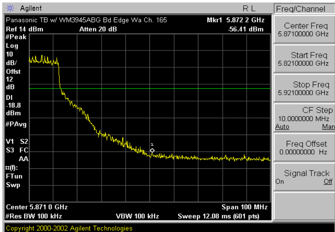
Plot 6-24. Band Edge Plot (802.11a – Ch. 165)
