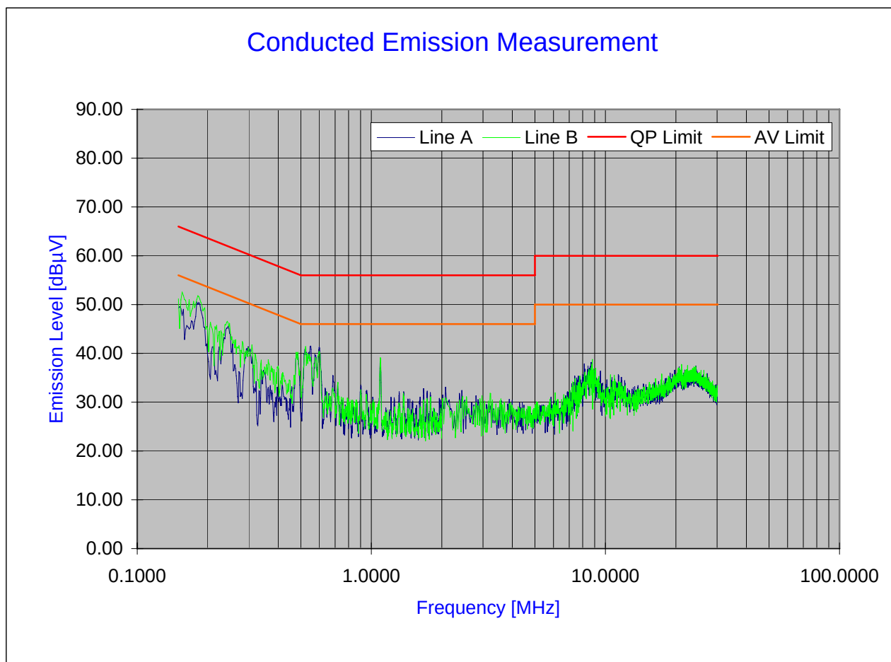
Plot 6-25. Line Conducted Plot with 802.11b with Docking Station
