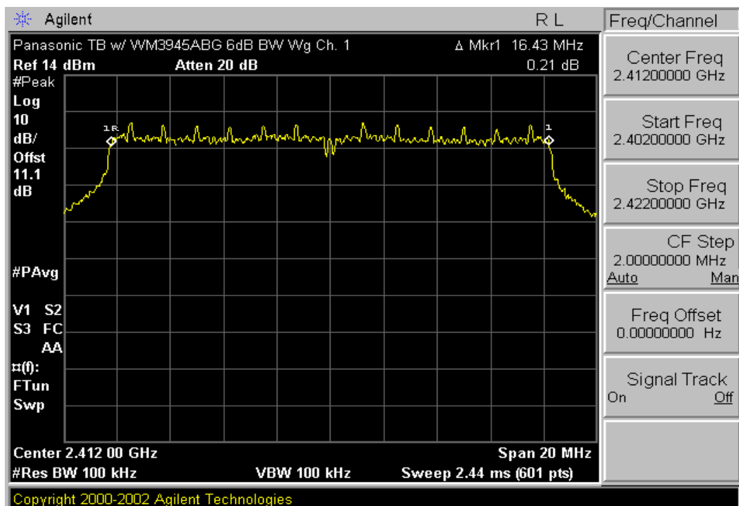
Plot 6-4. 6dB Bandwidth Plot (802.11g – Ch. 1)
