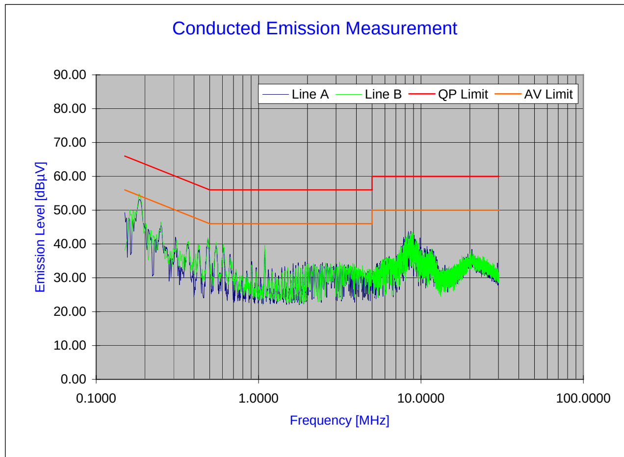
Plot 6-26. Line Conducted Plot with 802.11g with Docking Station
