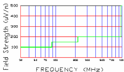
Figure 6-7. Radiated limits at 3 meters.
