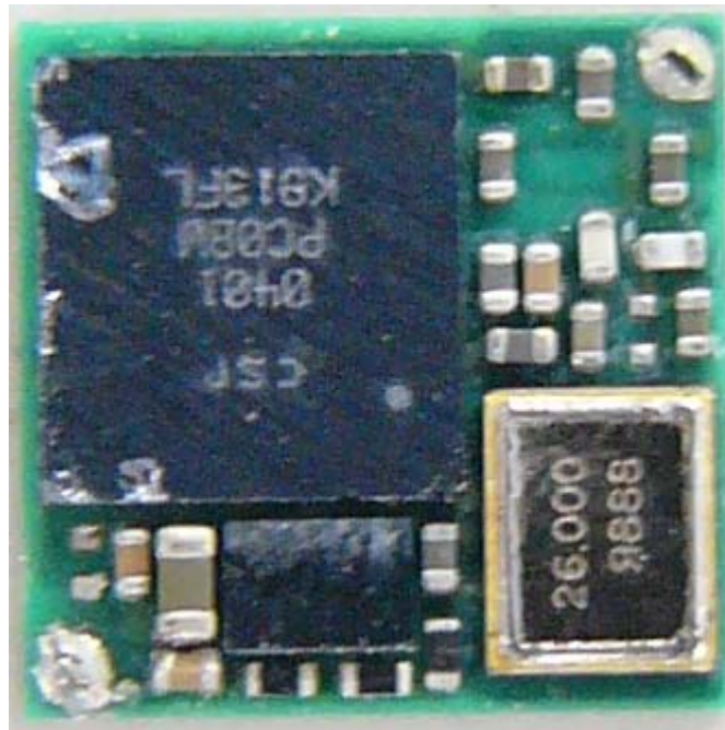
Bluetooth Module Top View (without shield plate)
