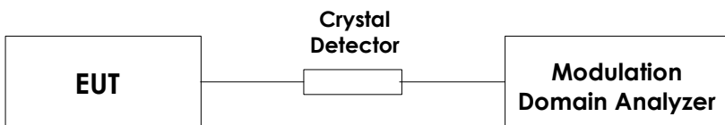
Test Set-up 2
