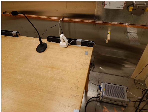
Power-Line Conducted Emissions, WX-ST600P
