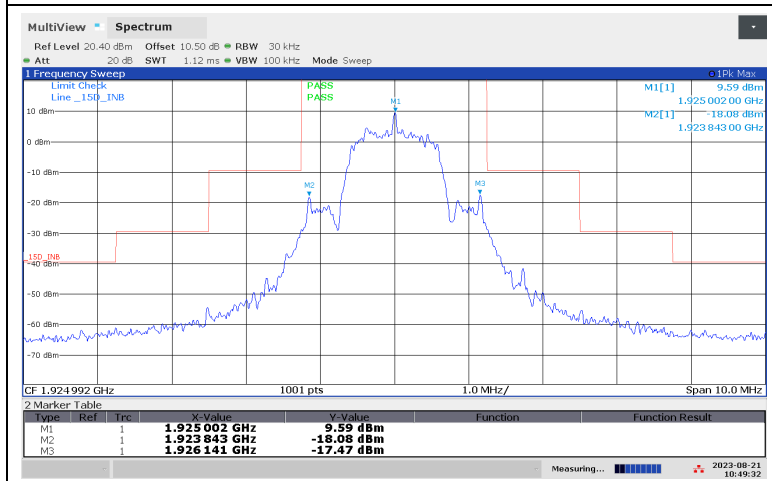
In-Band Unwanted Emissions, Middle Channel
