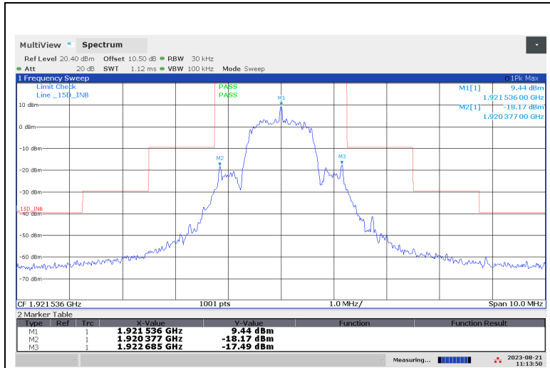
In-Band Unwanted Emissions, Lower Channel
