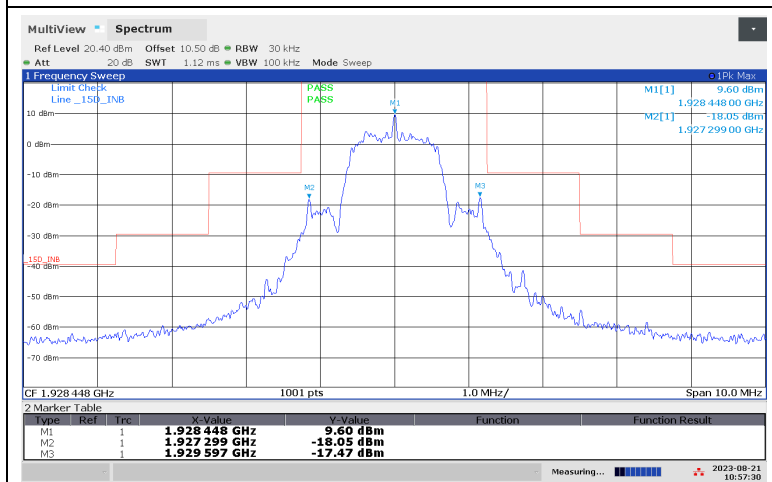
In-Band Unwanted Emissions, Upper Channel
