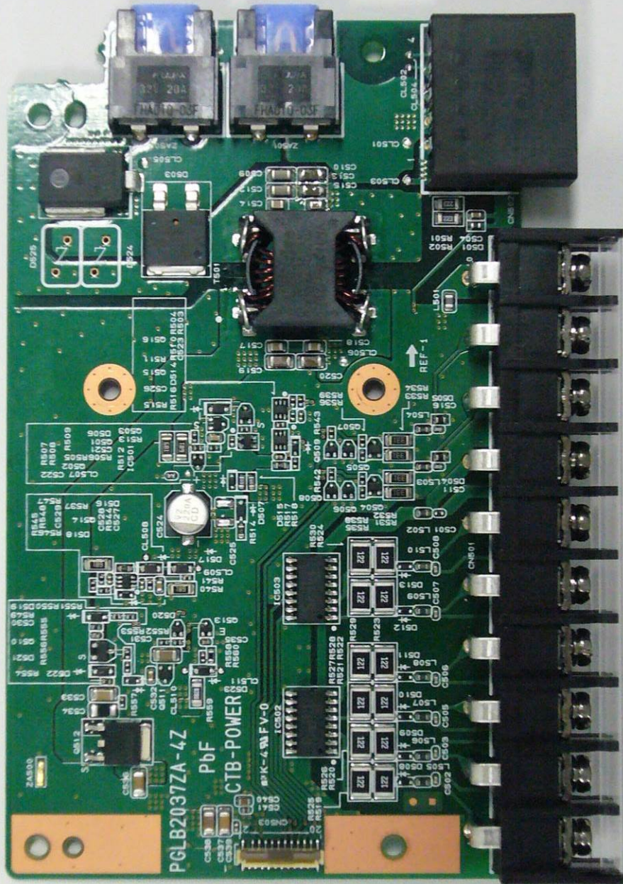
Power Board
