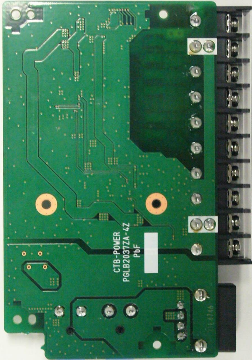
Back Side
