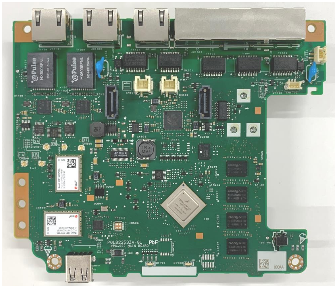
MAIN PCB Top View
