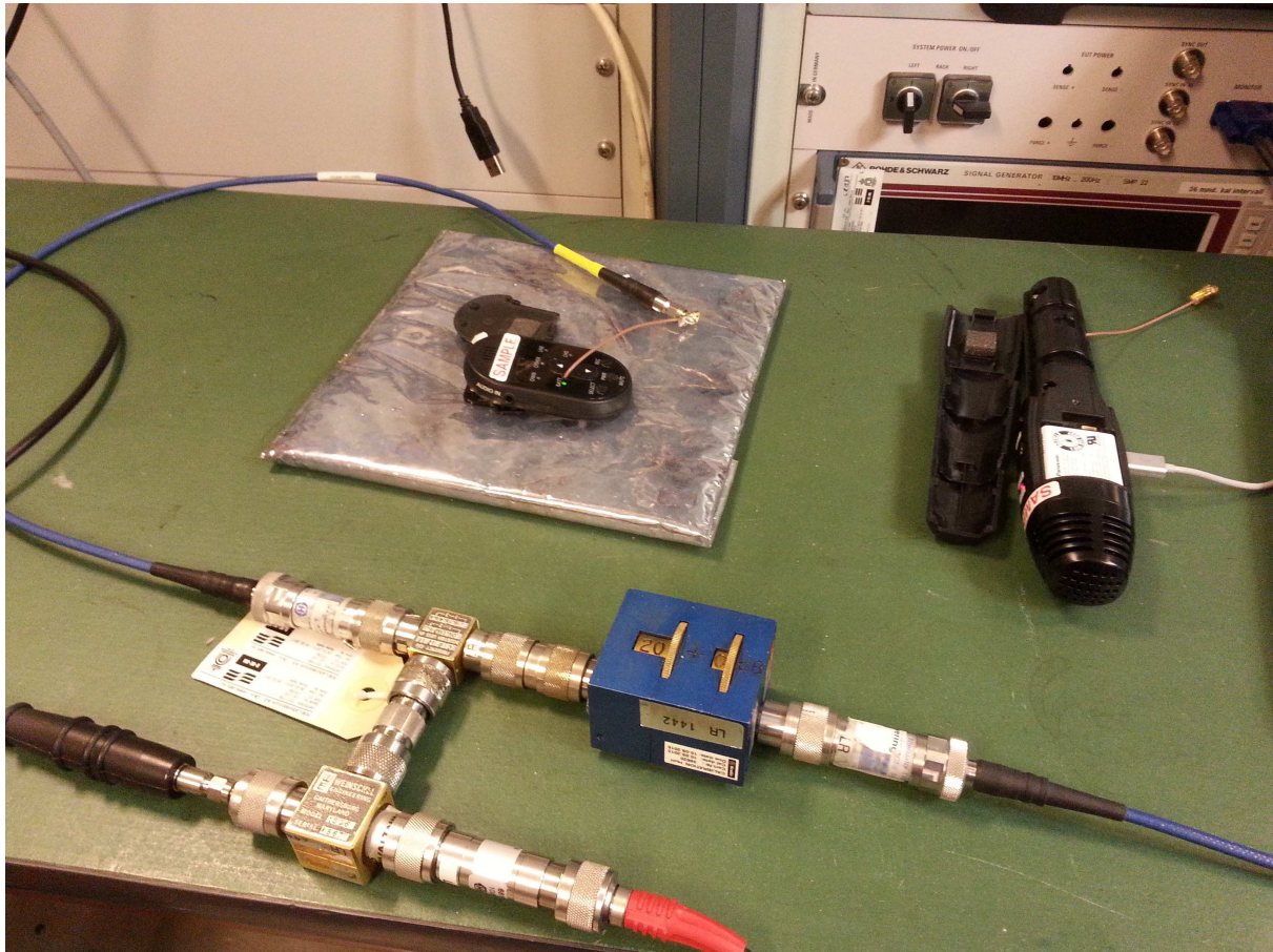
Conducted Test
