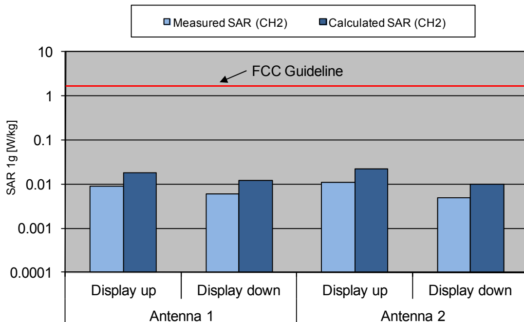
Fig. 9: The measured and calculated body phantom SAR values for the Panasonic KX-UDT131, antenna 1 and 2 for the US DECT standard in comparison to the FCC exposure limit.
