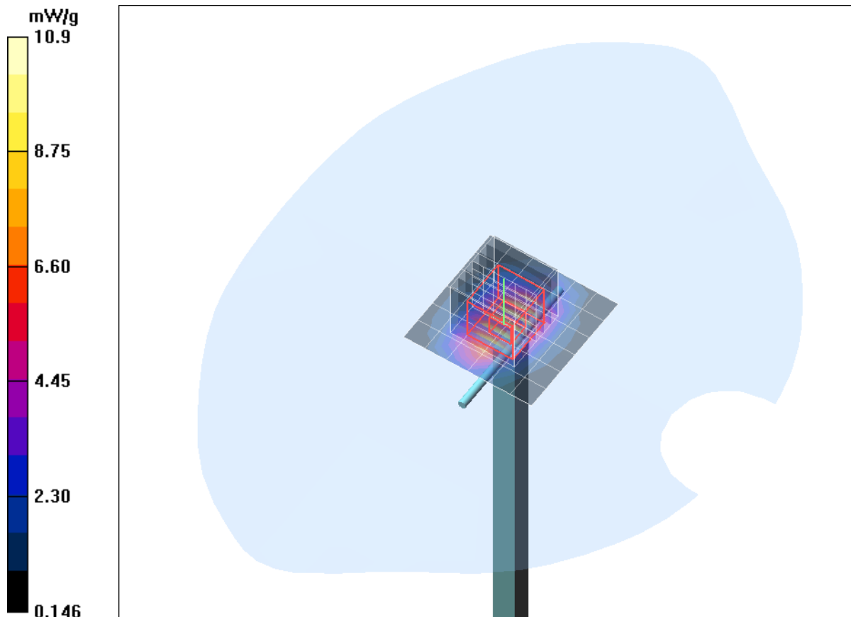
Fig. 10: Validation measurement 1900 MHz Head (October 23, 2012), coarse grid. Ambient Temperature: 22.0° C, Liquid Temperature: 21.9° C.
