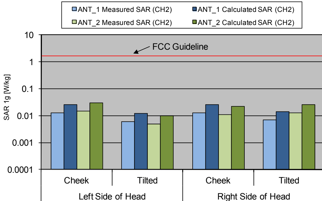
Fig. 8: The measured and calculated head phantom SAR values for the Panasonic KX-UDT131, antenna 1 and 2 for the US DECT standard in comparison to the FCC exposure limit.
