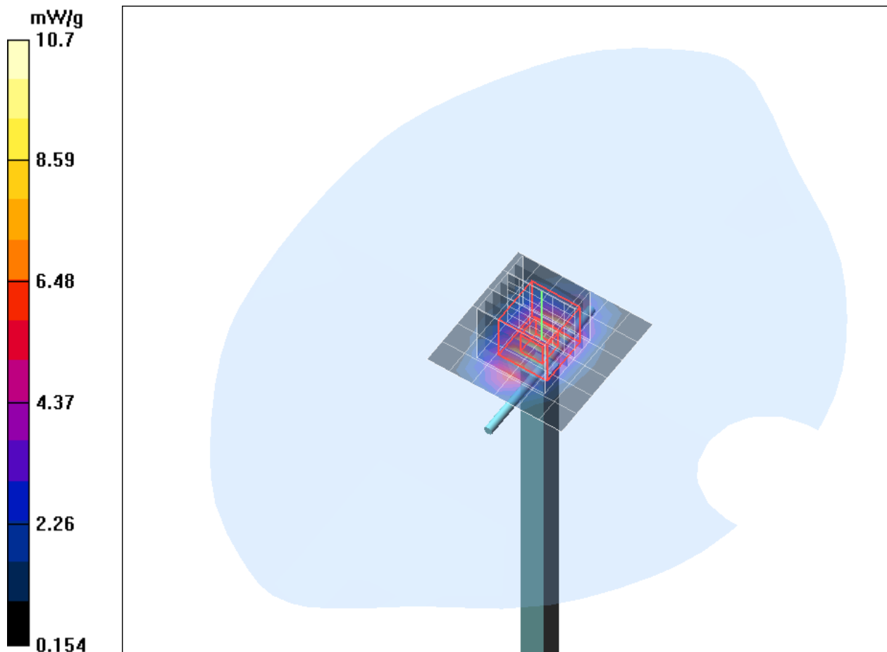
Fig. 11: Validation measurement 1900 MHz Body (November 16, 2012), coarse grid. Ambient Temperature: 22.0° C, Liquid Temperature: 21.8° C.
