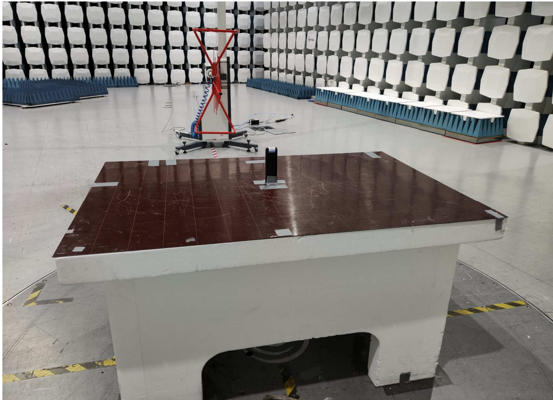
Radiated Emissions Below 1 GHz
