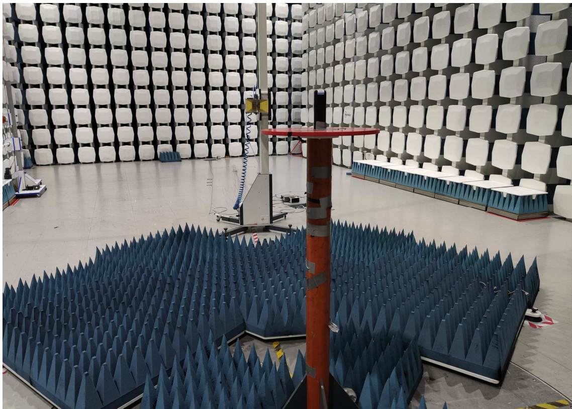
Radiated Emissions Above 1 GHz
