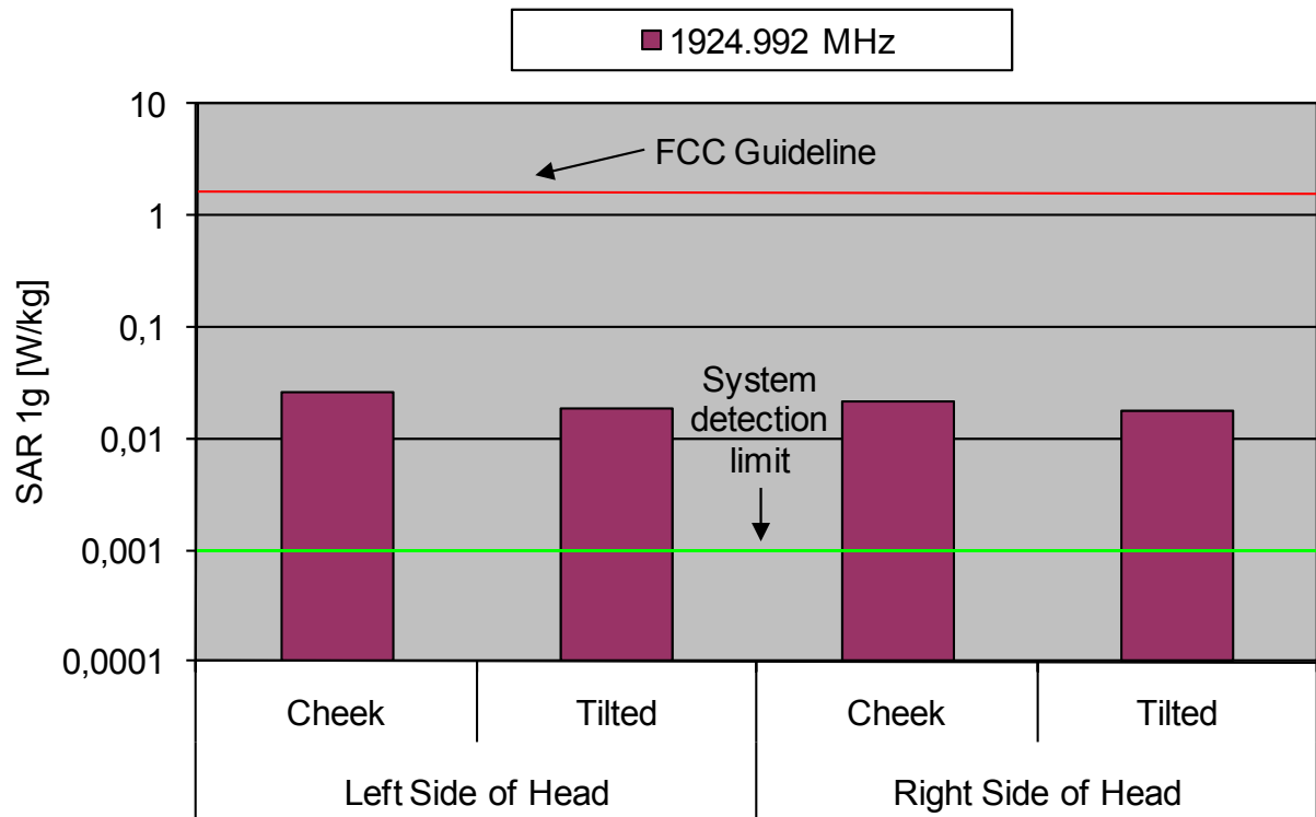
Fig. 8: The measured head phantom SAR values for the Panasonic KX-TGA410 for the US DECT standard in comparison to the FCC exposure limit.
