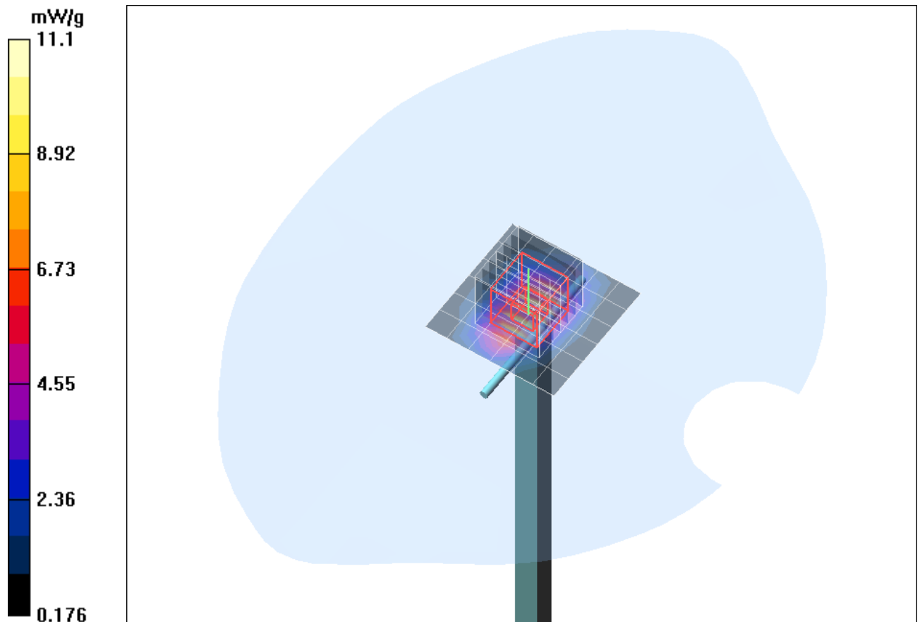
Fig. 9: Validation measurement 1900 MHz Head (November 26, 2010), coarse grid. Ambient Temperature: 21.0° C, Liquid Temperature: 20.8° C.
