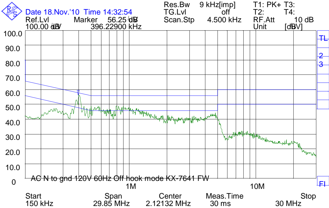
Phase N, Hook Off, AC Adaptor PNLV226(FW)
