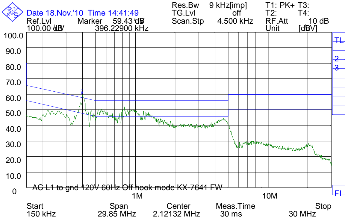
Phase L1, Hook Off, AC Adaptor PNLV226(FW)
