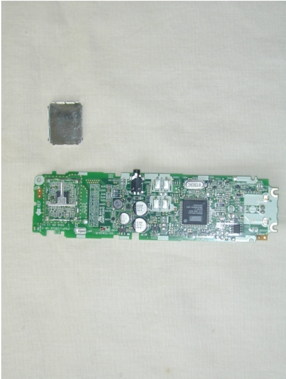
P.C. Board (RF Cover Open)
