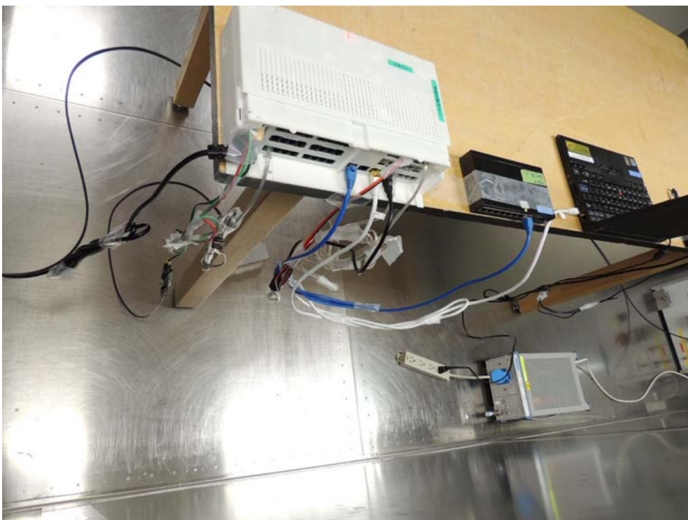
Photograph 9: Set-up for AC Power Line Conducted Emission of Transmitter, Rear View
