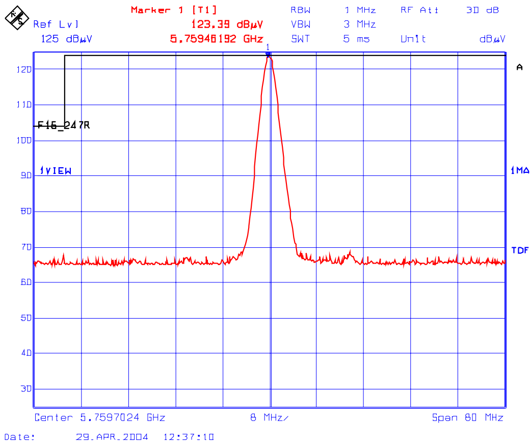
Plot 27: Band-Edge RF Radiated Emissions @ 3 meters Low End of Frequency Band Vertical Polarization
