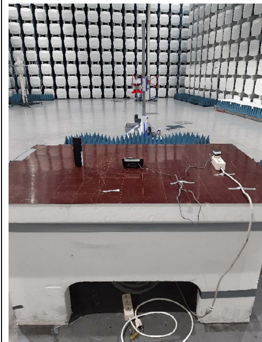
Handset and Base, Off-hook, Radiated emissions
