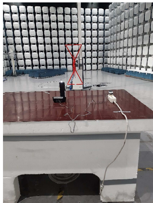
Handset and Base, On-hook, Radiated emissions
