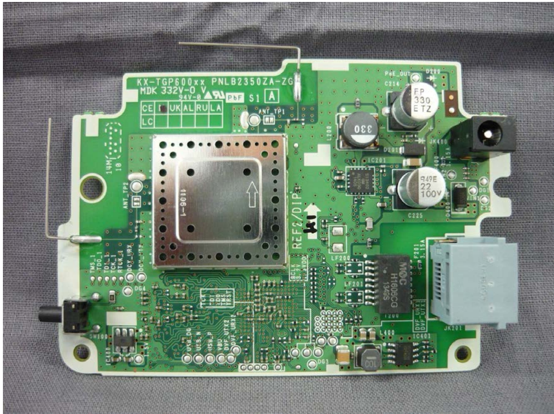
RF block under the shield case
