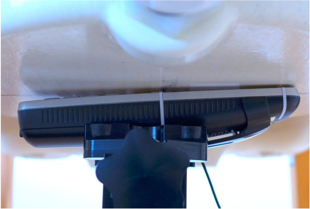
Pic. 8: Test position front side of EUT towards the phantom, 0 mm gap, belt clip and headset attached.
