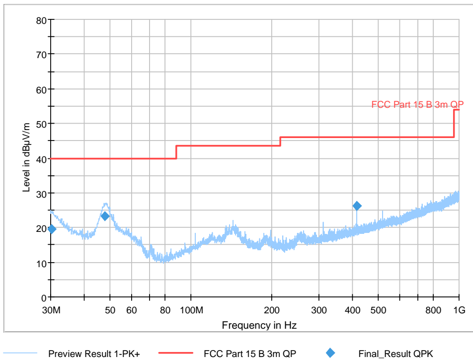
Radiated Emissions 30 – 1000 MHz, AC Adaptor PNLV223 (2C)
