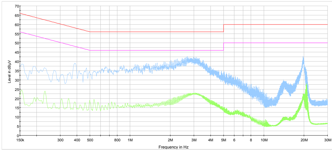
Panasonic KX-TGFA61 _ 120V 60Hz Neutral — CISPR 32 Mains O-Peak Class B Limit — CISPR 32 Mains Average Class B Limit — Preview Result 1-PK+ — Preview Result 2-AVG
