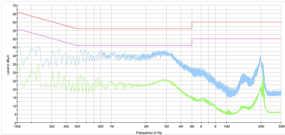
Panasonic KX-TGFA61 _ 120V 60Hz Phase — CISPR 32 Mains O-Peak Class B Limit — CISPR 32 Mains Average Class B Limit — Preview Result 1-PK+ — Preview Result 2-AVG
