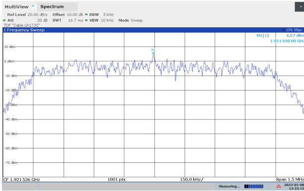
PSD Overview, Lower Channel
