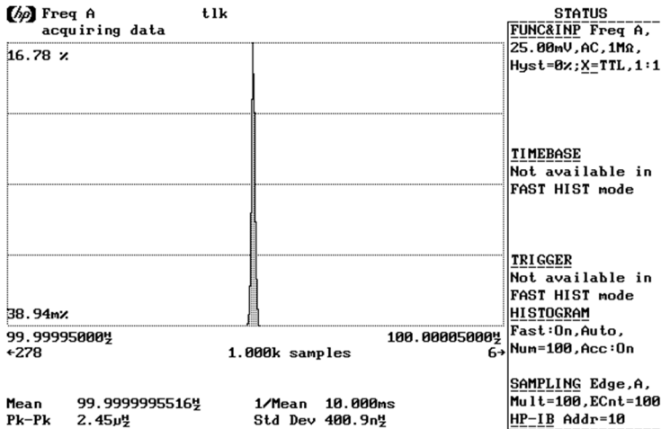
Frame Repetition Stability, Gated over 100 Frames
