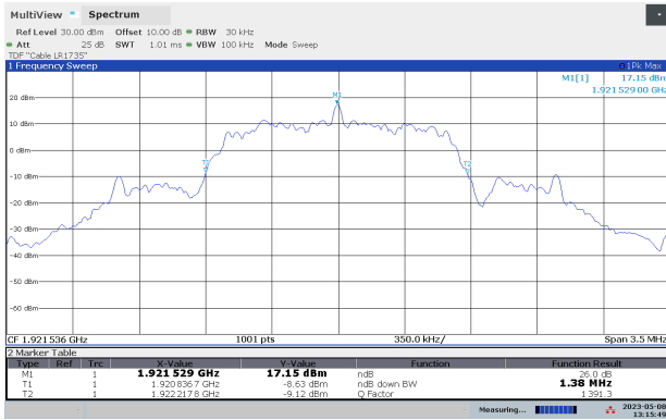
Emission Bandwidth B, Lower Channel
