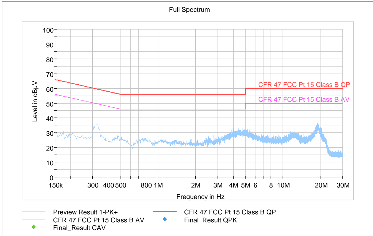
Active Call, 120V 60Hz
