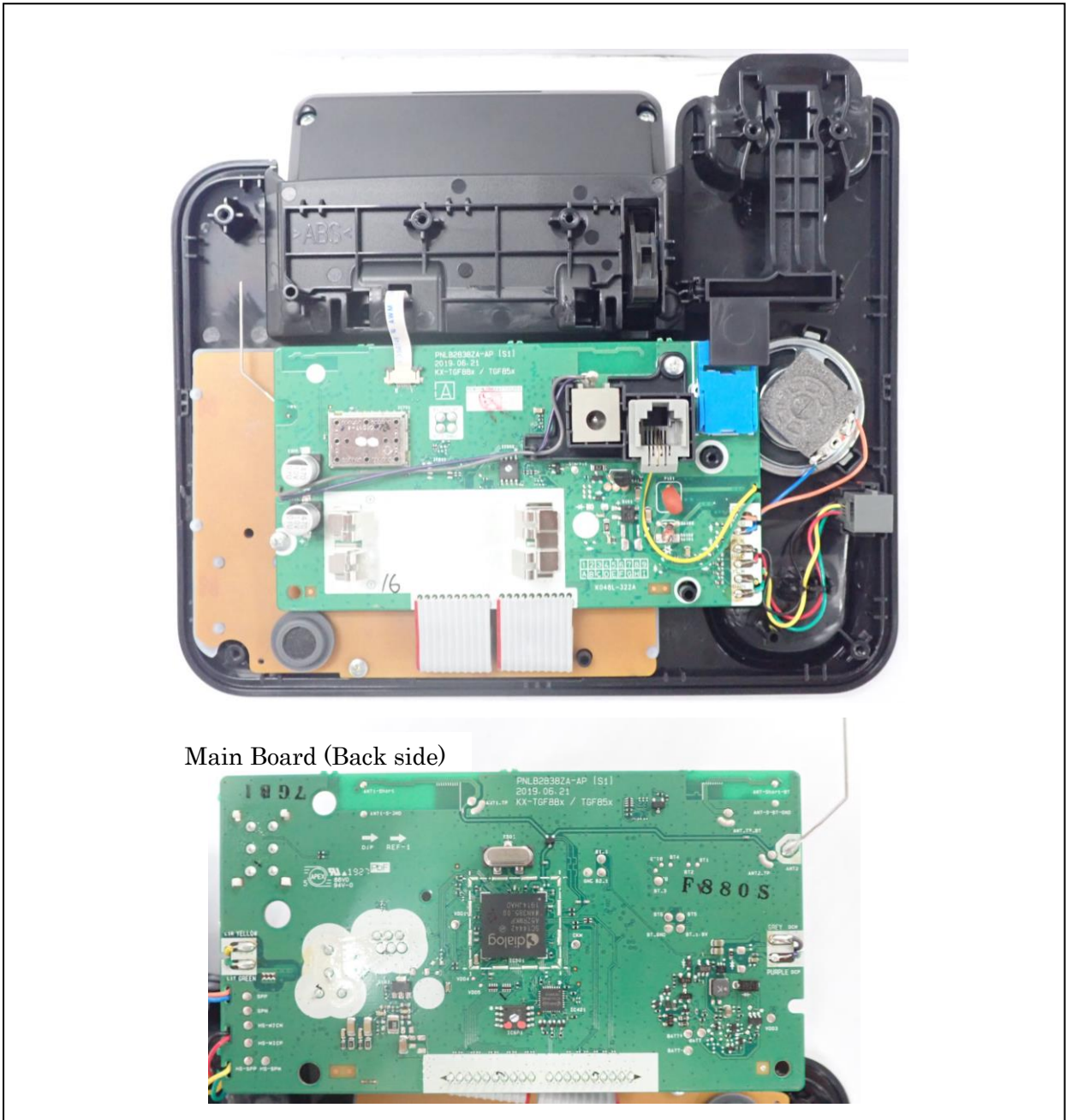
Internal View
