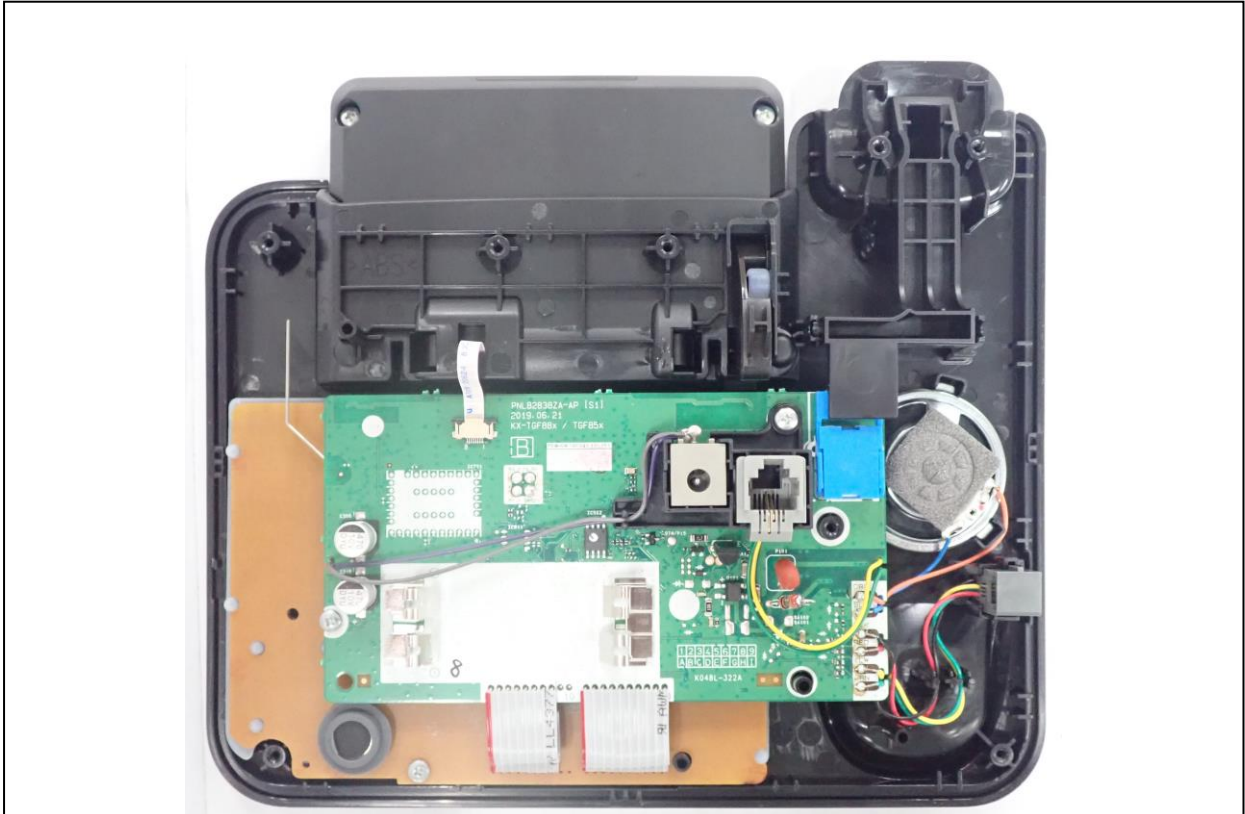
Main Board (Back side)
