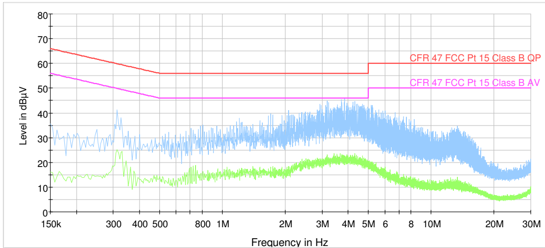
120V 60Hz, OFF Hook
