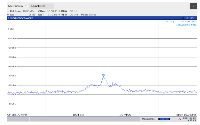
Spurious 165.77 MHz, Upper Channel
