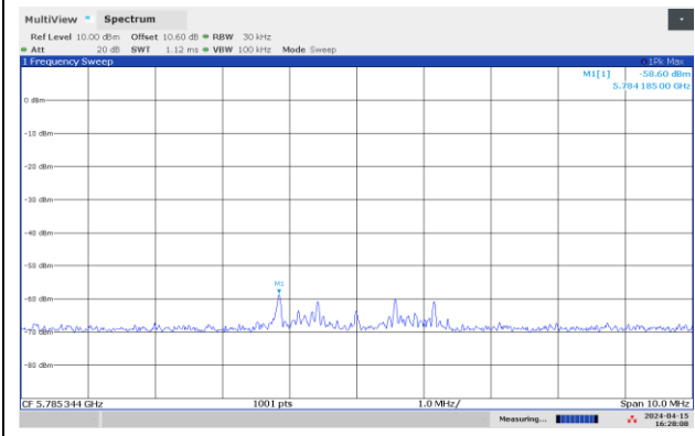
Spurious 5785 MHz, Upper Channel
