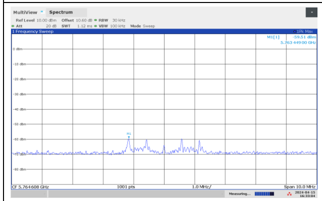
Spurious 5765 MHz, Lower Channel
