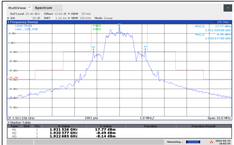
In-Band Unwanted Emissions, Lower Channel
