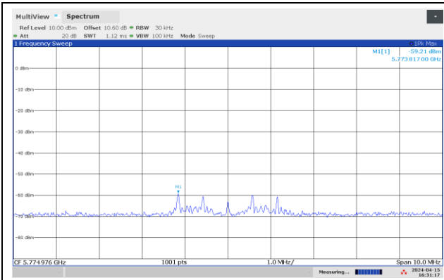
Spurious 5775 MHz, Middle Channel
