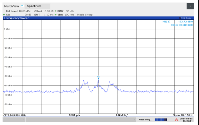
Spurious 3850 MHz, Middle Channel
