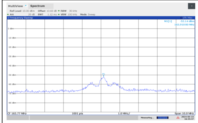
Spurious 165.77 MHz, Middle Channel
