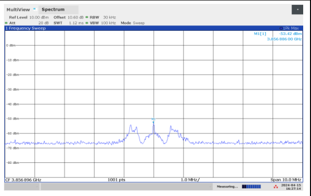
Spurious 3857 MHz, Upper Channel
