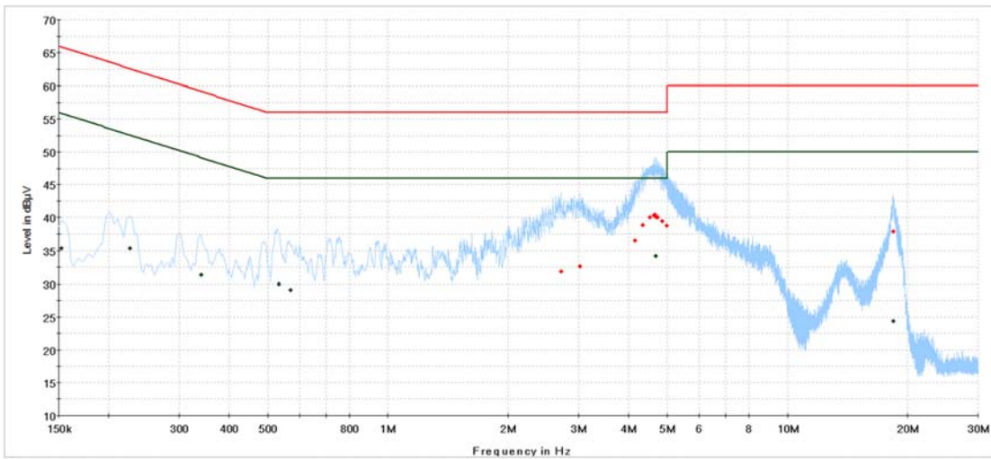
CE - TGEA 60 charging Phase Preview Result 1-PK + CISPR 22 Mains Q-Peak Class B Limit CISPR 22 Mains Average Class B Limit Final_Result QPK Final_Result CAV
