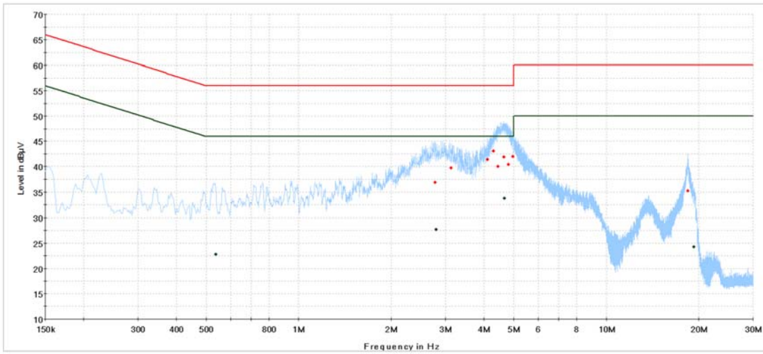
CE - TGEA 60 charging Neutral Preview Result 1-PK + CISPR 22 Mains Q-Peak Class B Limit CISPR 22 Mains Average Class B Limit Final_Result QPK Final_Result CAV
