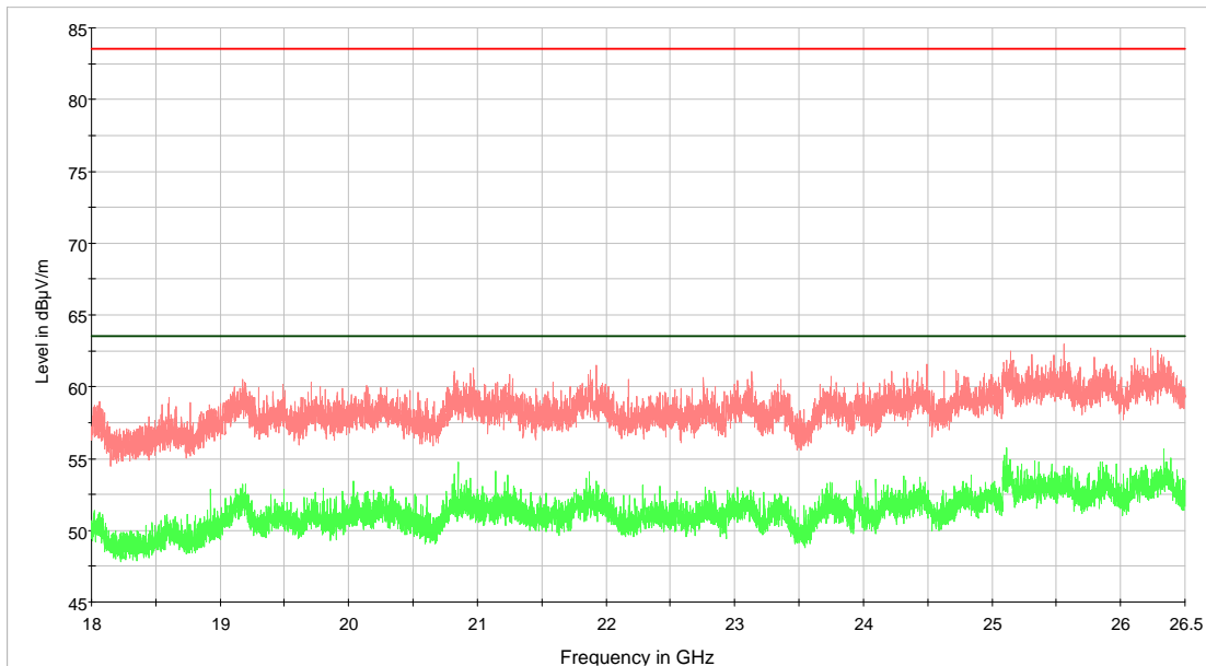
RE 18 to 26.5 GHz TGE670 [middle channel] — AVG_MAXH — PK+_MAXH — FCC Part 15 and ICES- Class B 1m Peak Limit — FCC Part 15 and ICES - Class B 1m Average Limit
