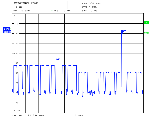
EUT Transmits on Free RECEIVE Slot, AFTER
