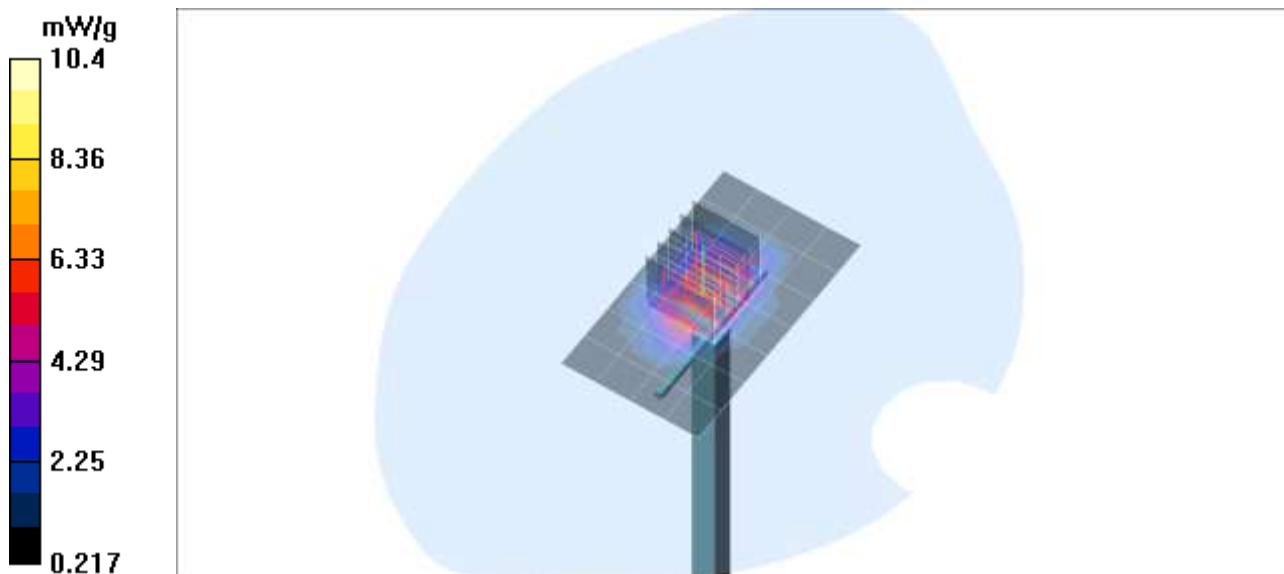
Plot. 3: SAR Verification Measurement 1900 MHz (November 17, 2021).
