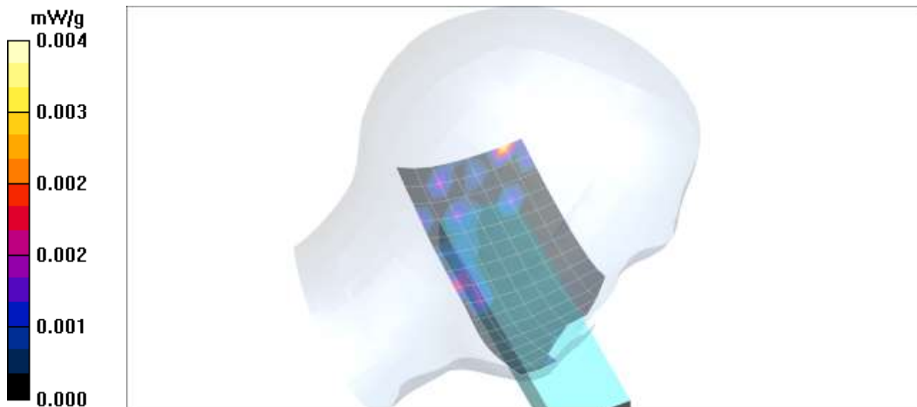
Plot. 2: SAR distribution plot for BT, channel 39, head configuration, left cheek.
