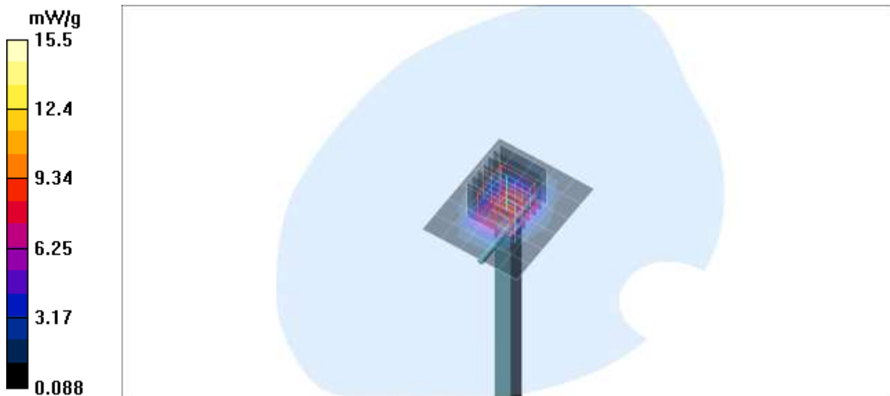
Plot. 4: SAR Verification Measurement 2450 MHz (December 07, 2021).
