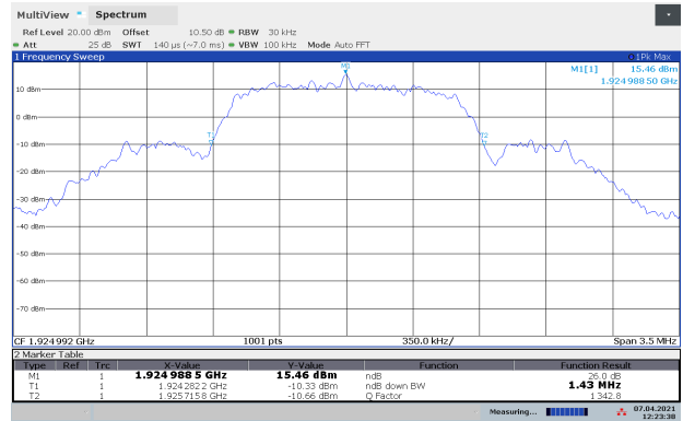
Emission Bandwidth B, Middle Channel
