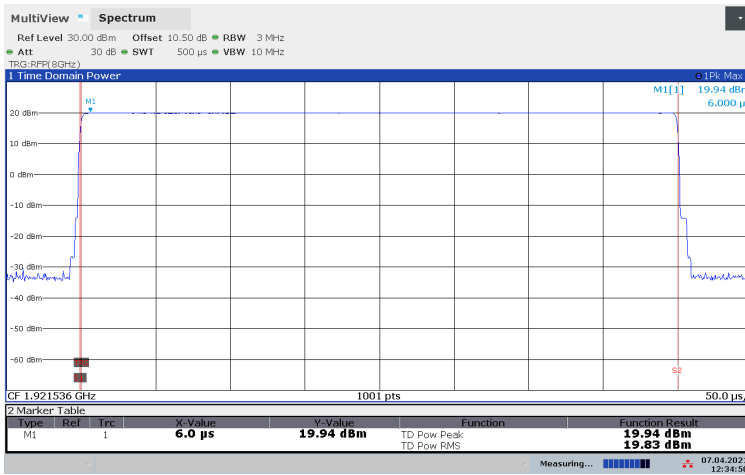
Conducted Peak Output Power, Lower Channel
