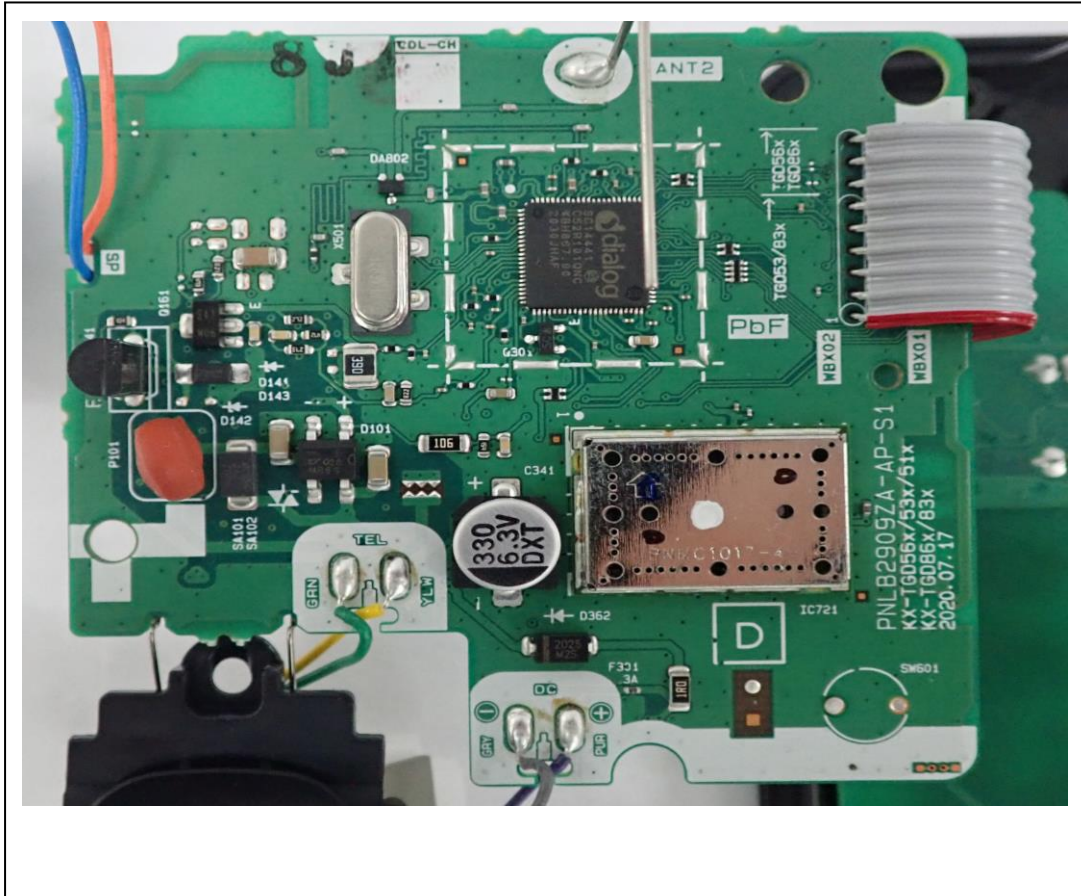
Main Board
