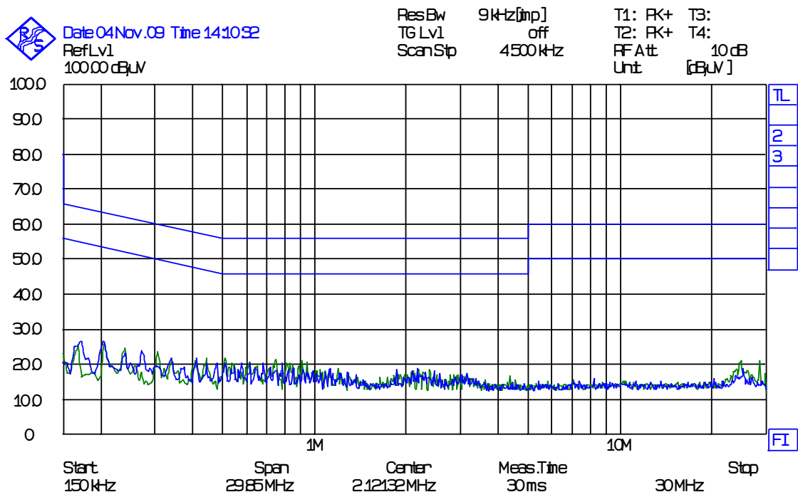
In charger, charging, charger #4, Phase N and L1
