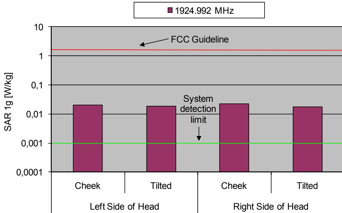
Fig. 8: The measured head phantom SAR values for the Panasonic KX-TGA660 for the US DECT standard in comparison to the FCC exposure limit.
