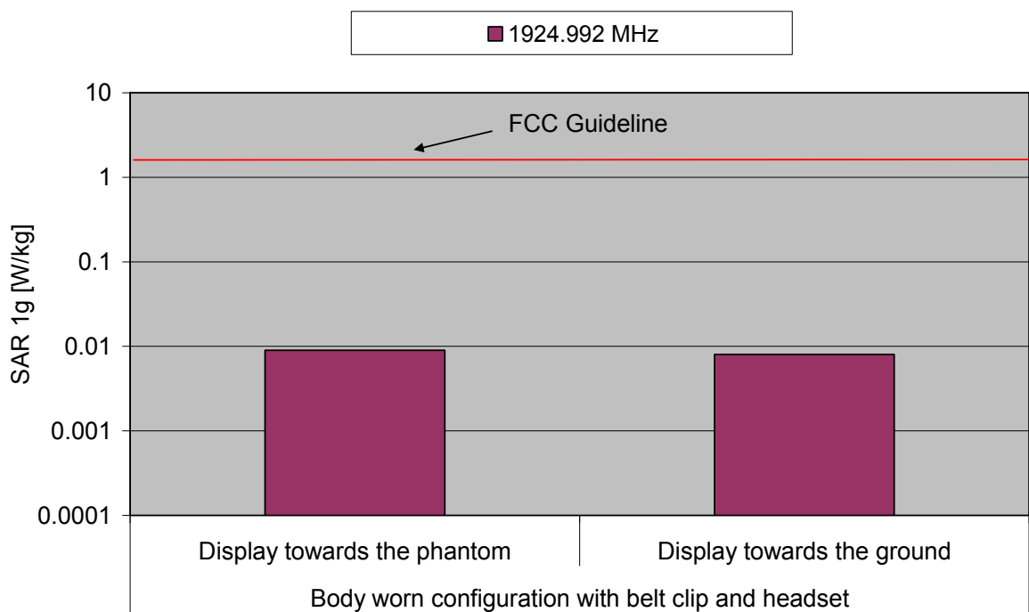
Fig. 9: The measured SAR values in body-worn configuration for the Panasonic KX-TGA651 for the US DECT standard in comparison to the FCC exposure limit.
