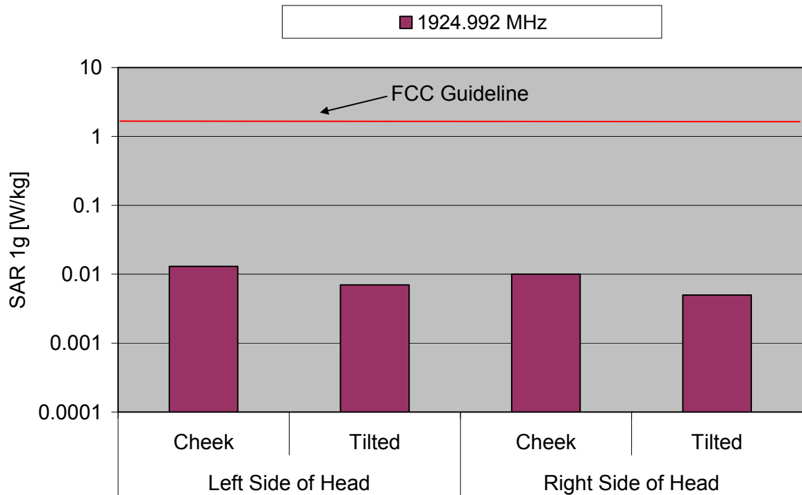
Fig. 8: The measured head phantom SAR values for the Panasonic KX-TGA651 for the US DECT standard in comparison to the FCC exposure limit.
