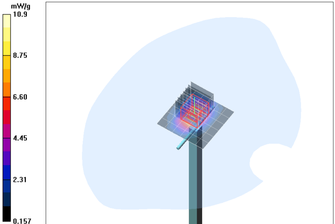
Fig. 10: Validation measurement 1900 MHz Head (November 13, 2009), coarse grid. Ambient Temperature: 22.1° C, Liquid Temperature: 21.6° C.
