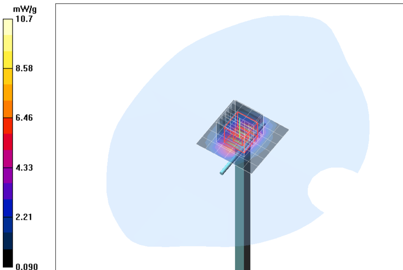
Fig. 9: Validation measurement 1900 MHz Head (December 08, 2011), coarse grid. Ambient Temperature: 22.0° C, Liquid Temperature: 21.6° C.
