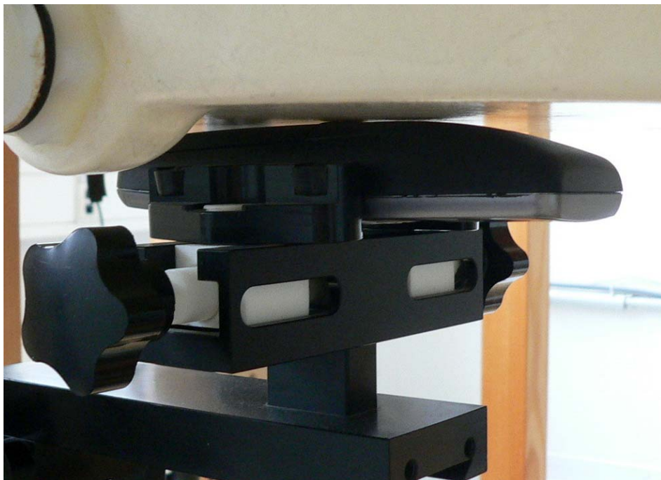
Fig. 19: Body worn configuration for KX-TGA277, position 2, display towards the ground, 0 mm distance.
