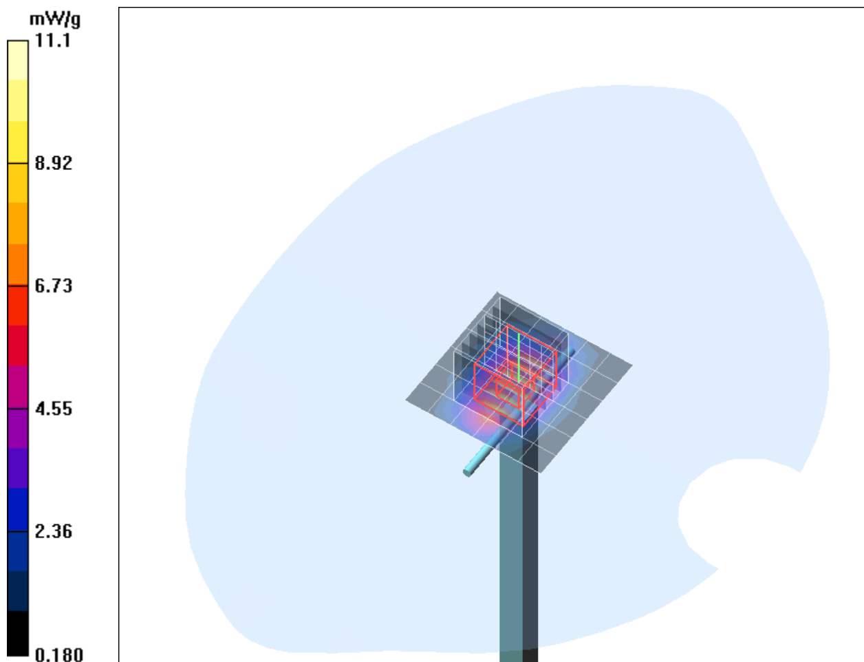
Fig. 10: Validation measurement 1900 MHz Body (July 10, 2013), coarse grid.
