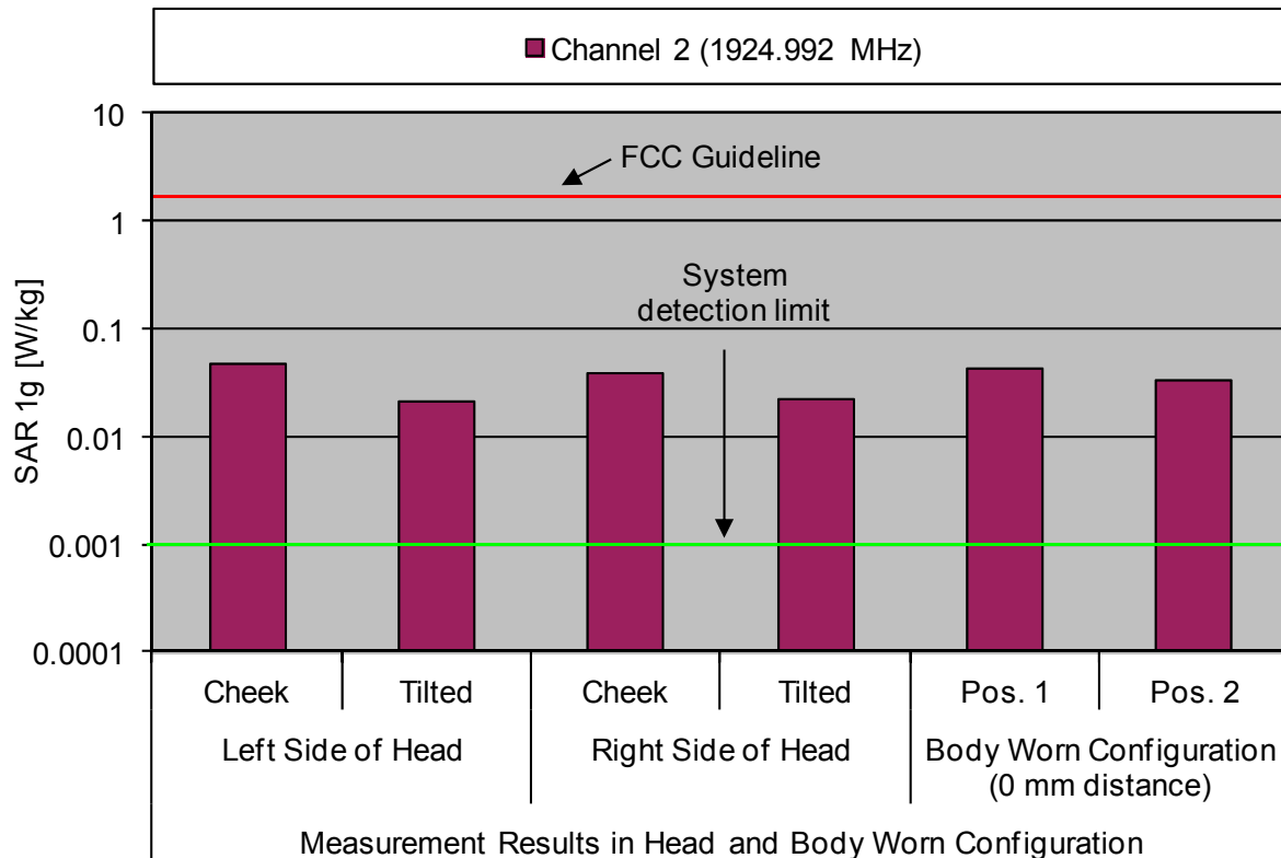
Fig. 8: The reported SAR values for head and body worn configuration for the Panasonic KX-TGA277, for the US DECT standard in comparison to the FCC exposure limit.
