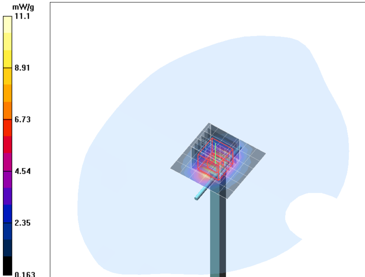
Fig. 9: Validation measurement 1900 MHz Head (July 10, 2013), coarse grid.
