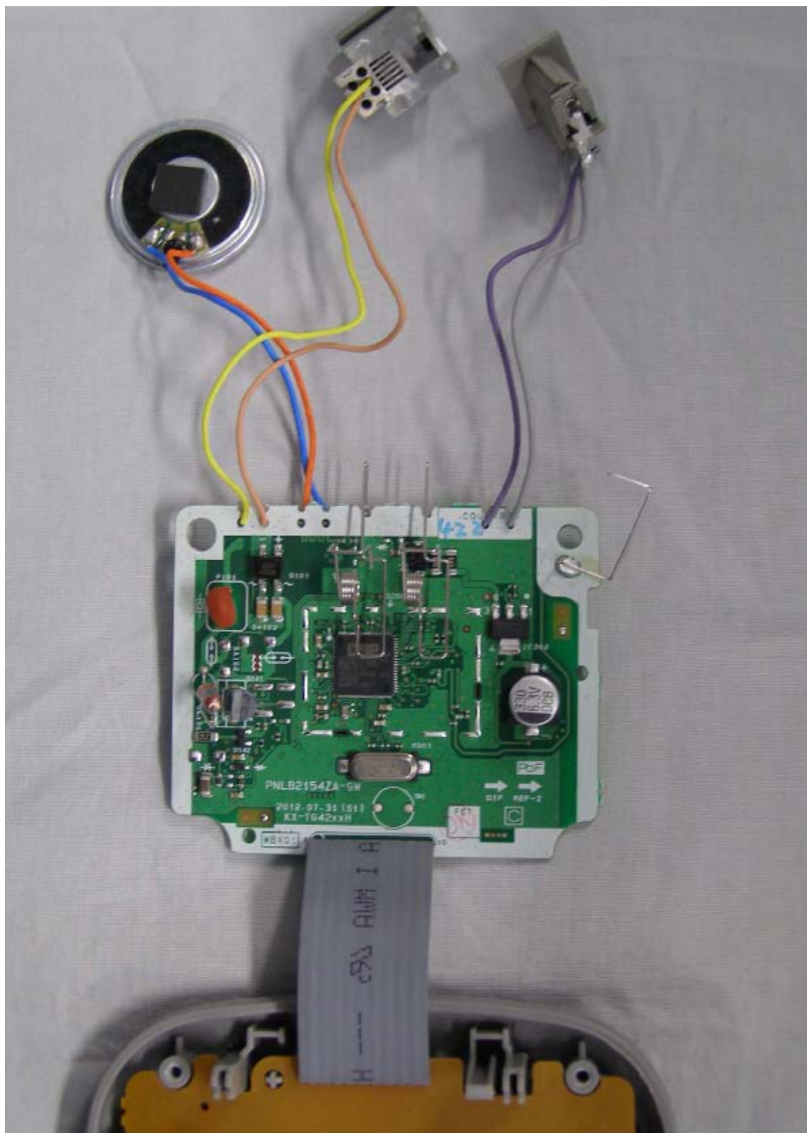
Main Board
