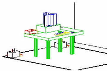
Figure 3. Wooden Table & Bonded LISNs
