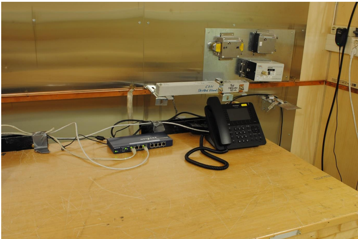
Conducted Emissions Test
