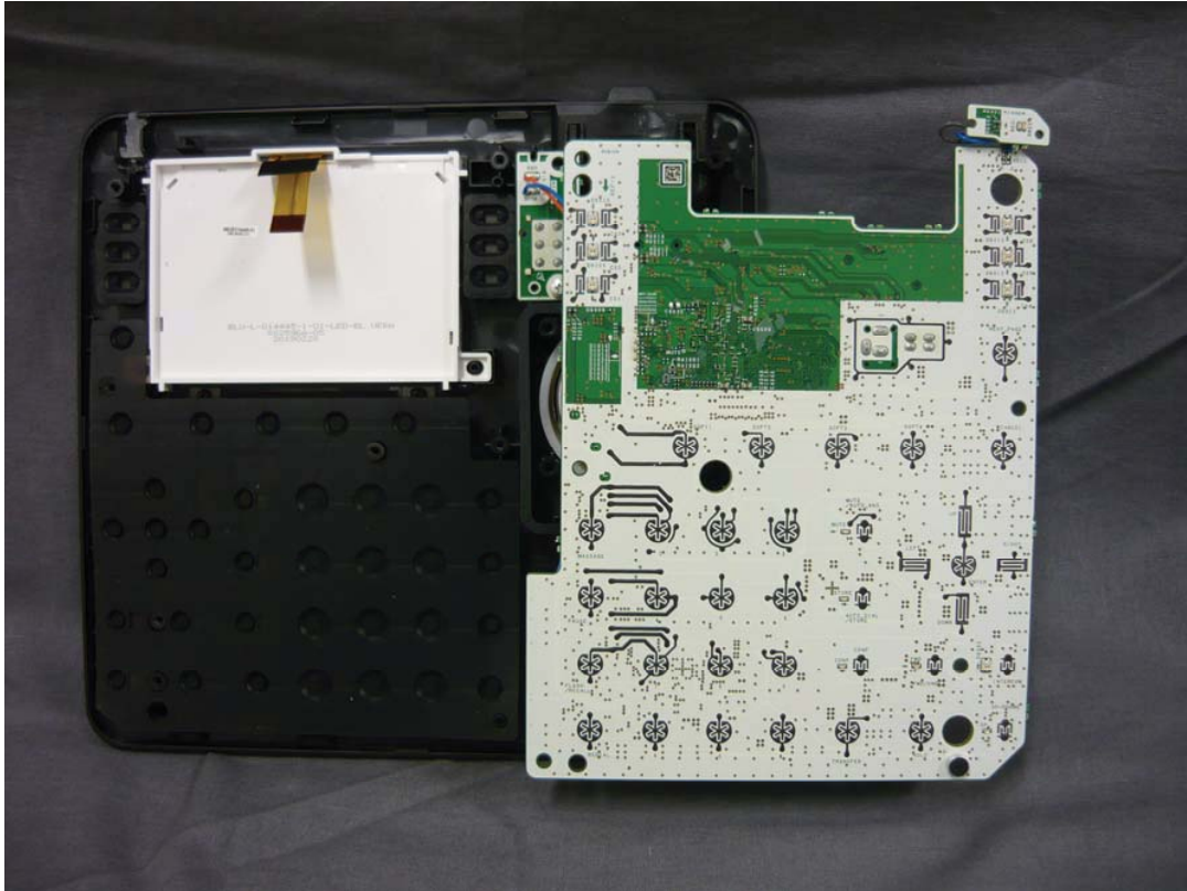
Fig.7 Internal view (Print board rear side)
