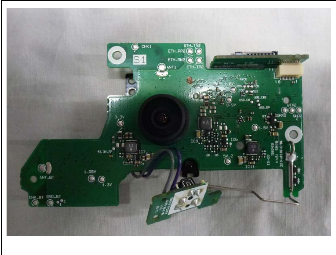
Main Board (The other side)
