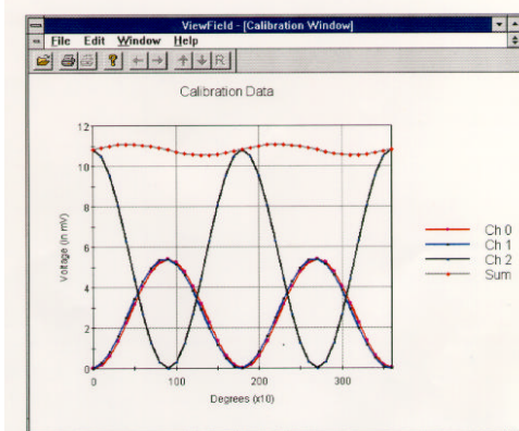
Figure 26 ViewField Calibration Window showing Probe Calibration Data
