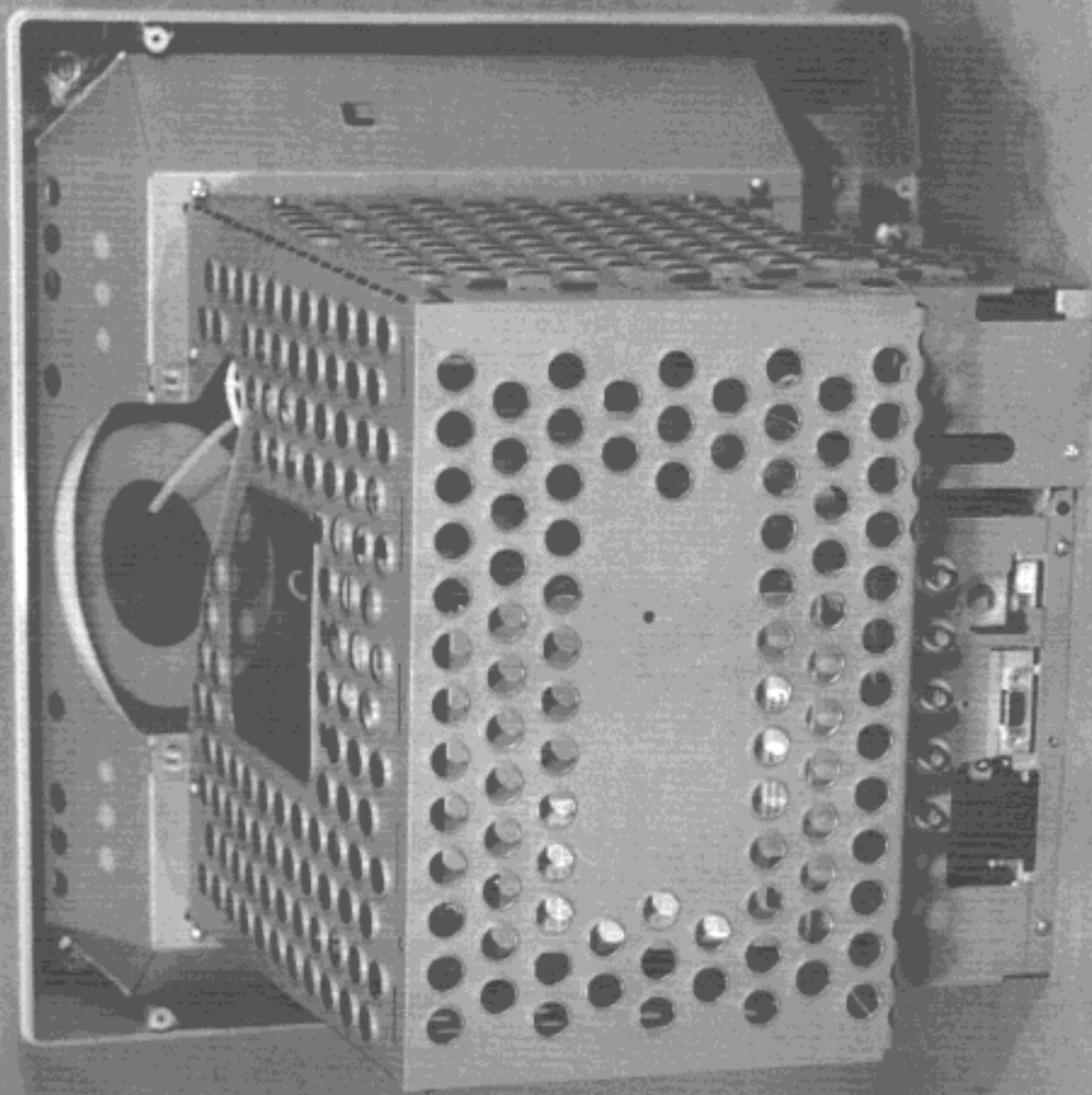
Photo 2. Inside view with shield case of TX-M9T55
