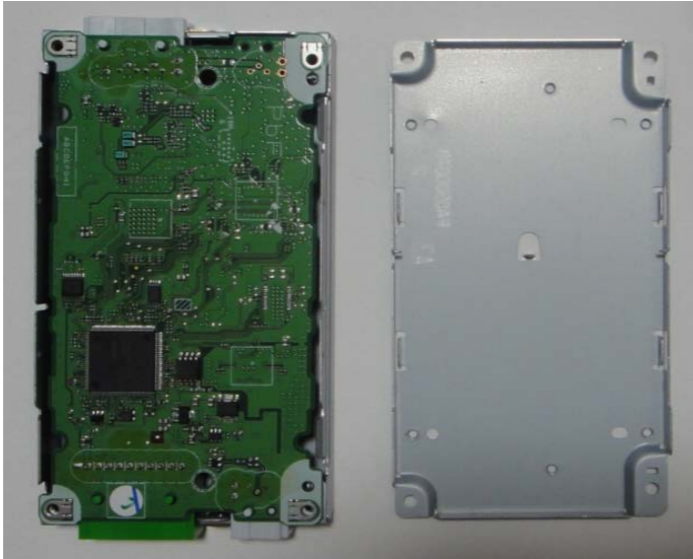
Inside of Unit (Ver.2)
