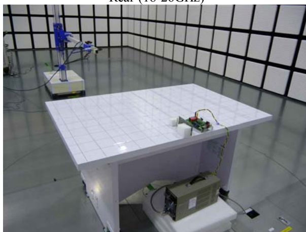
Rear (18-26GHz)
